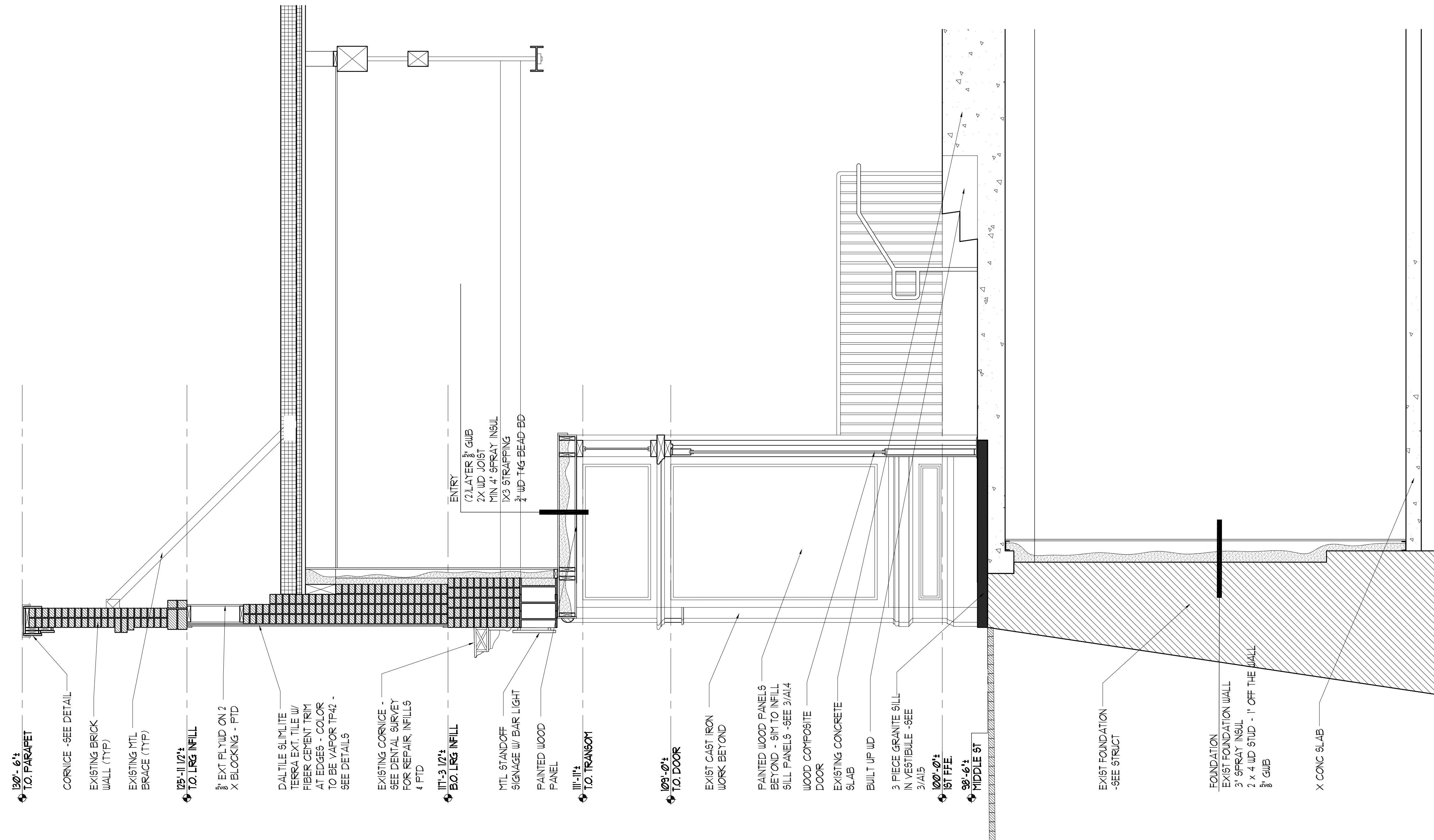
WALL SECTION @ FRONT ENTRY SCALE: 1/2" = 1'-0"
